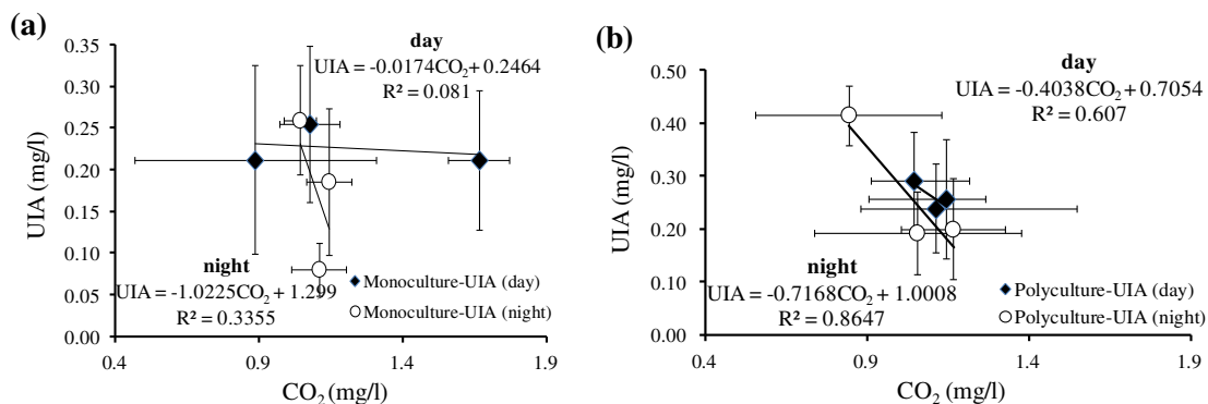
Fig. 4 Relationship between the levels of UIA (mg/l) and CO 2 (mg/l) during the day and night under a monoculture and b polyculture conditions
